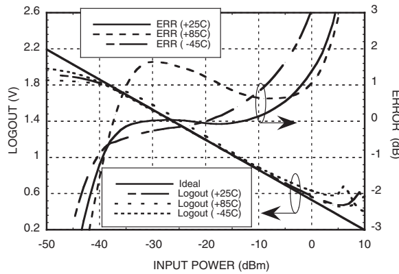
LOGOUT Voltage & Error vs. Input Power, f_{in} = 10000 MHz
